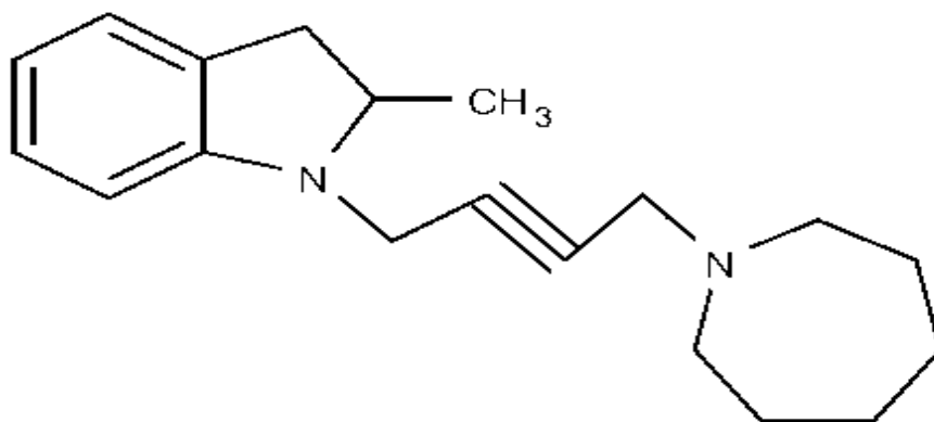
AZ-7: 1-[4-(azepan-1-yl)but-2-yn-1-yl]-2-methyl-2,3-dihydro-1H-indole.
