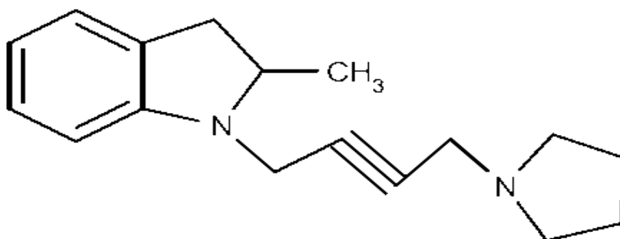
AZ-6: 2-methyl-1-[4-(pyrrolidin-1-yl)but-2-yn-1-yl]-2,3-dihydro-1H-indole.
