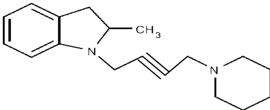
AZ-5: 2-methyl-1-[4-(piperidin-1-yl)but-2-yn-1-yl]-2,3-dihydro-1H-indole.
